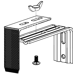
Bracket
