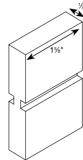
Z-Frame Buildout
