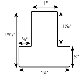
Standard T-Post
