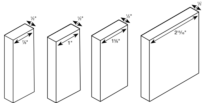
Sidelight Buildout
