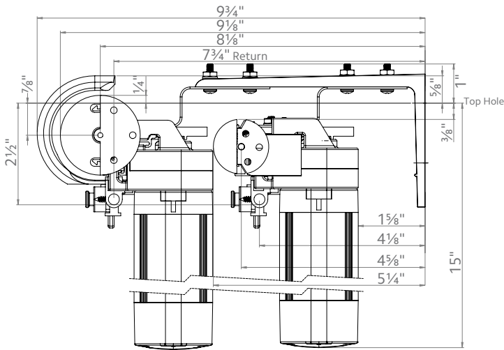
2" & 1 3/8" DOUBLE MOUNT
