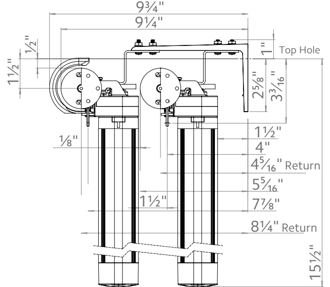
2" DOUBLE MOUNT
