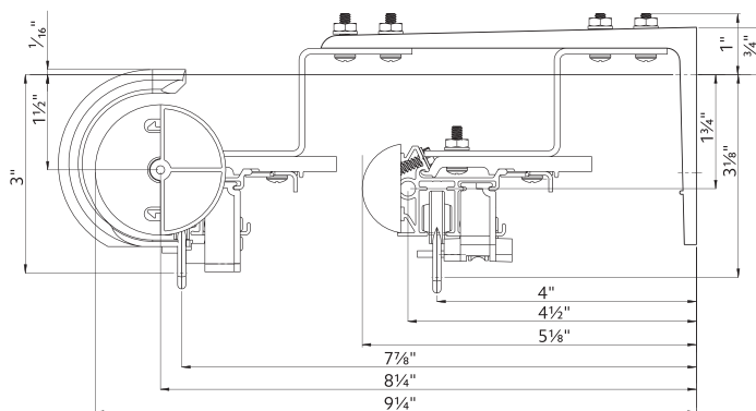
2" & 1 3/8" DOUBLE MOUNT
