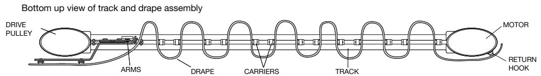
Bottom up view of track and drapery assembly
