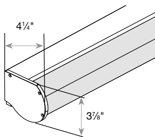
Medium Cassette Valance 1 3/4" Minimum Inside Mount
