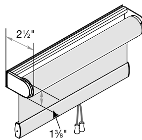
No Valance* 2" Minimum Inside Mount
