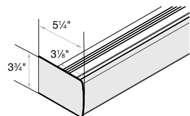
Contour Valance 2" Minimum Inside Mount (return can be trimmed)
