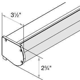
Small Cassette Valance 1 1/2" Minimum Inside Mount
