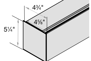
Flat Valance 2 15/16" Minimum Inside Mount (return can be trimmed)
