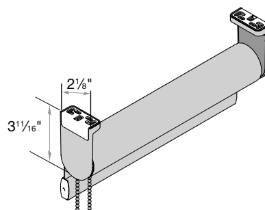
No Valance* Minimum Inside/Top Mount is equal to \frac{1}{2} the roll diameter, plus 1\frac{1}{2}"
