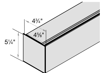
Flat Valance 2\frac{15}{16}" Minimum Inside Mount (return can be trimmed)
