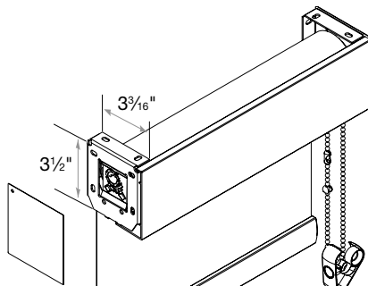
3" Fascia 2\frac{3}{4}" Minimum Inside/Top Mount \frac{3}{4}" Minimum Inside/Side Mount
