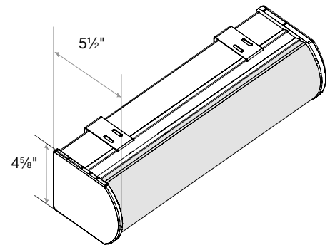
Large Cassette Valance 1\frac{1}{4}" Minimum Inside Mount
