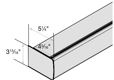
Contour Valance 3\frac{1}{2}" Minimum Inside Mount (return can be trimmed)
