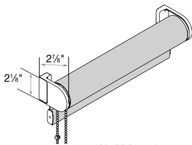
No Valance* \frac{3}{4}" Minimum Inside/Side Mount
