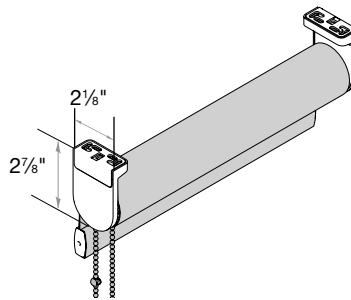
No Valance* Minimum Inside/Top Mount is equal to \frac{1}{2} the roll diameter, plus 1\frac{1}{2}"
