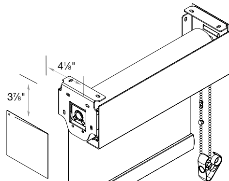
4" Fascia 3\frac{3}{4}" Minimum Inside/Top Mount 1\frac{1}{2}" Minimum Inside/Side Mount
