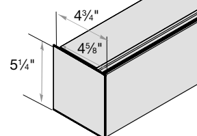
Flat Valance 2 15/16" Minimum Inside Mount (return can be trimmed)
