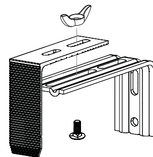
Bracket
