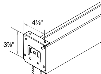
4" Fascia 3 3/4" Minimum Inside/Top Mount 1 1/2" Minimum Inside/Side Mount
