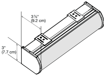
Small Cassette Valance 1 1/8" (3.5 cm) Minimum Inside Mount
