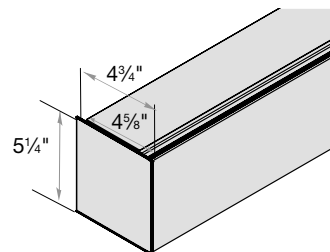
Flat Valance 2\frac{15}{16}" Minimum Inside Mount (return can be trimmed)
