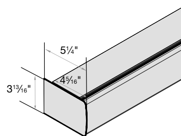
Contour Valance 3\frac{1}{2}" Minimum Inside Mount (return can be trimmed)
