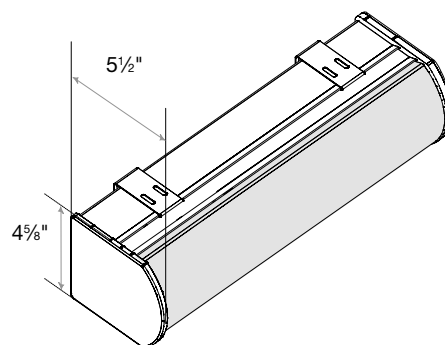
Large Cassette Valance 1\frac{1}{4}" Minimum Inside Mount
