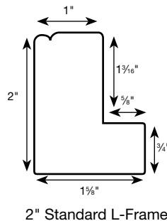
2" Standard L-Frame
