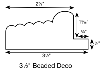
3 1/2" Beaded Deco
