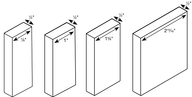
Sidelight Buildout
