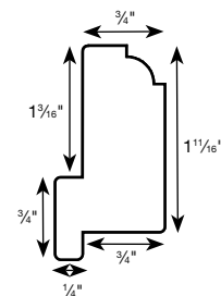
Tilt-Out Z-Frame
