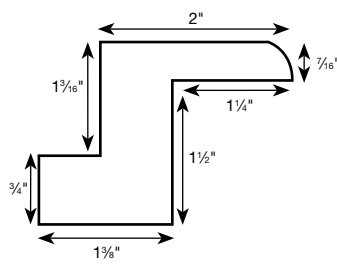
Bullnose Z-Frame
