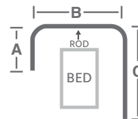
Cubicle Style 3: J-Track
