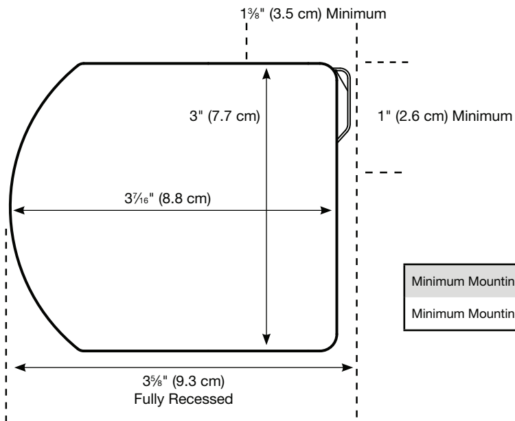
Fabric-Wrapped Cassette
