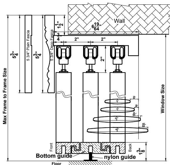
Semi-Inside Mount
