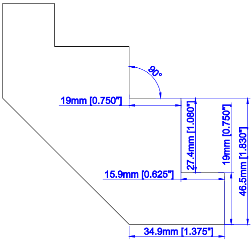
2" Sill Plate
