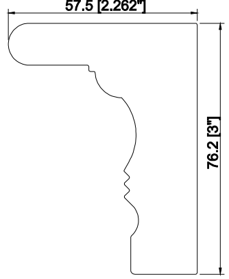
3" Sill Frame
