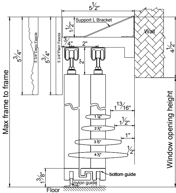
Outside Mount
