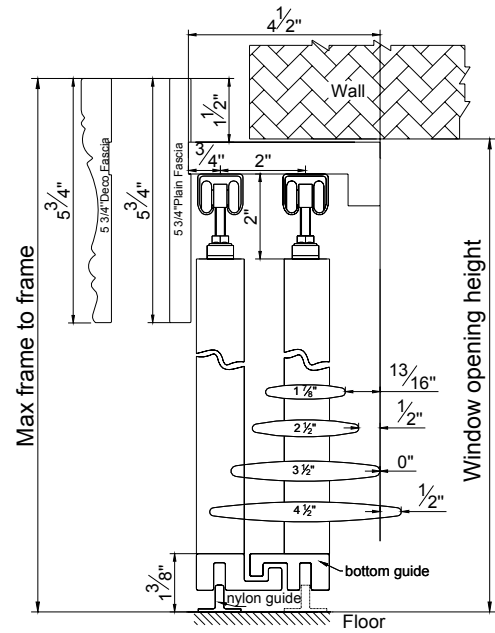
Semi-Inside Mount
