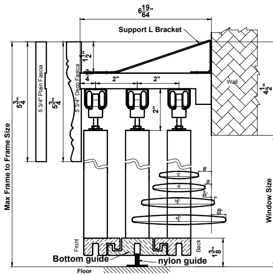
Outside Mount
