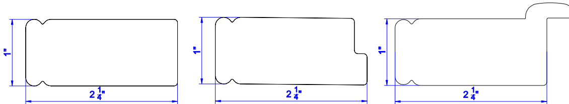
2 1/4" Butt Stile
