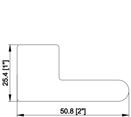
2" Sill Plate
