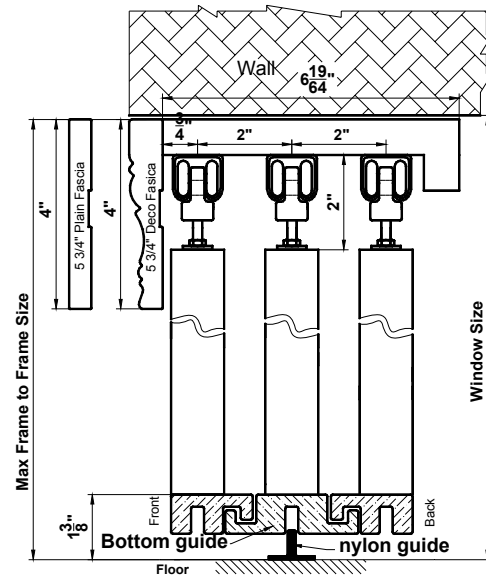
Inside Mount
