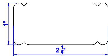
2 1/4" Center Stile
