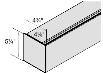
Flat Valance 2\frac{15}{16}" Minimum Inside Mount (return can be trimmed)
