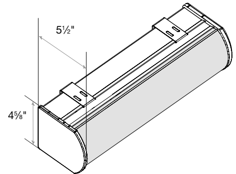
Large Cassette Valance 1\frac{1}{4}" Minimum Inside Mount
