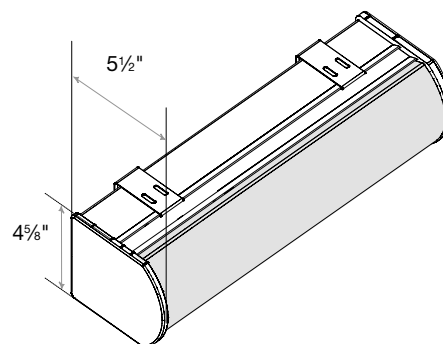
Large/Dual Cassette Valance 1 3/4" Minimum Inside Mount
