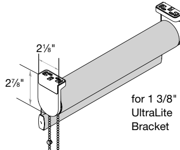
No Valance* Minimum Inside/Top Mount is equal to \frac{1}{2} the roll diameter, plus 1\frac{1}{2}"
