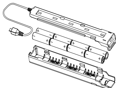
Battery Case (non-rechargeable solution) Dimensions: 9 1/4" x 1 1/4" x 7/8"
