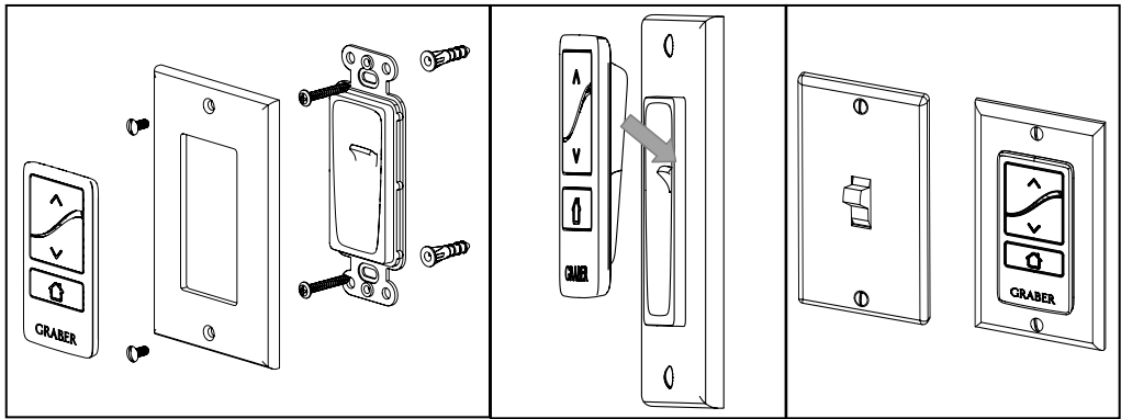
Optional Decorator Wall Plate Mount (see options for details)
