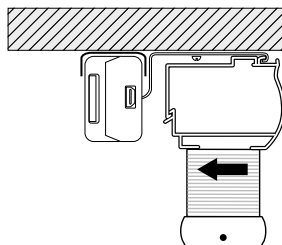
Ceiling/Inside Mount
