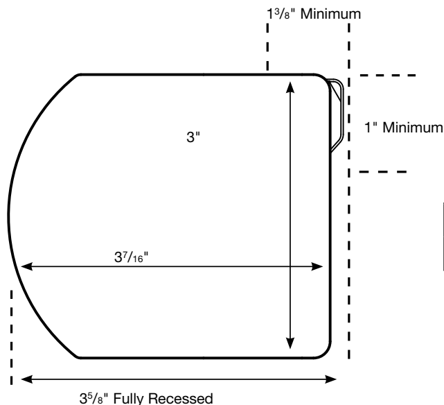
Fabric-Wrapped Cassette
